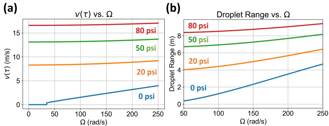
Figure 12. Effect of p init on v(\tau) and droplet range. The p init values presented are of 0 psi (no pinit), 20 psi, 50 psi and 80 psi. Parameters used for plotting are h_0=25 mm, l=70 mm, \phi=60^\circ and a=4 mm. (a) Plot of v(\tau) vs. \Omega shows that a larger p init leads to a larger v(\tau) by providing an initial flow velocity at the inlet. The variation of v(\tau) with \Omega declines with p init . (b) Relationship of droplet range vs. \Omega shows that larger p init leads to a larger droplet range. The variation of droplet range with \Omega is significant.
