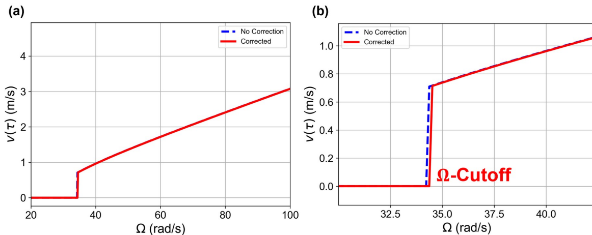
Figure 6. Theory v - \Omega plot with (solid red) and without (dashed blue) the correction of fluid effects. The line is plotted with the parameters h_0=25 mm, l=7.0 cm, a=2 mm, \phi=60 degrees. (a) The two curves are nearly indistinguishable. (b) Zooming in into the \Omega -cutoff region reveals that the cutoff angular velocity is larger after the correction, though the effect of such correction at angular velocities above the cutoff is insignificant.
